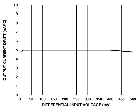
Figure 9. Output Current Drift vs. Differential Input Voltage
