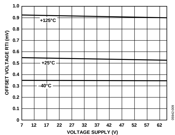
Figure 8. Input Offset Voltage vs. Supply (Pin V+)
