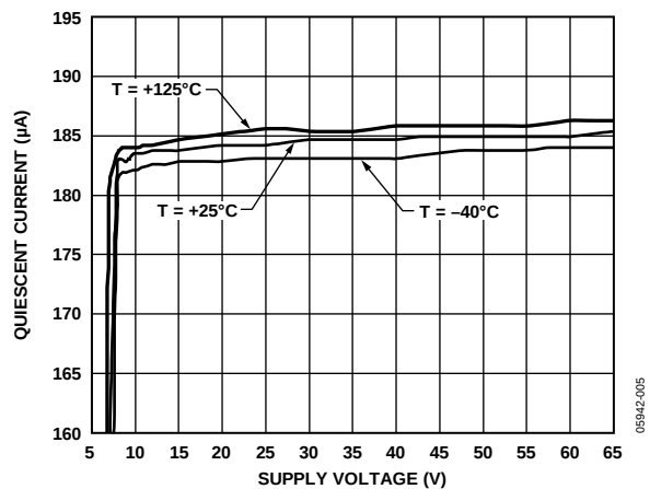
Figure 4. Supply Current vs. Supply (Pin V+) ( I_{OUT} = 0 mA)
