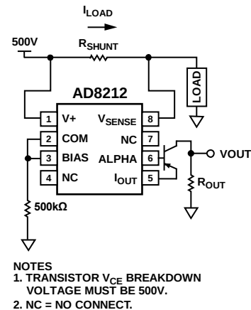
Figure 26. High Voltage Operation Using External PNP
