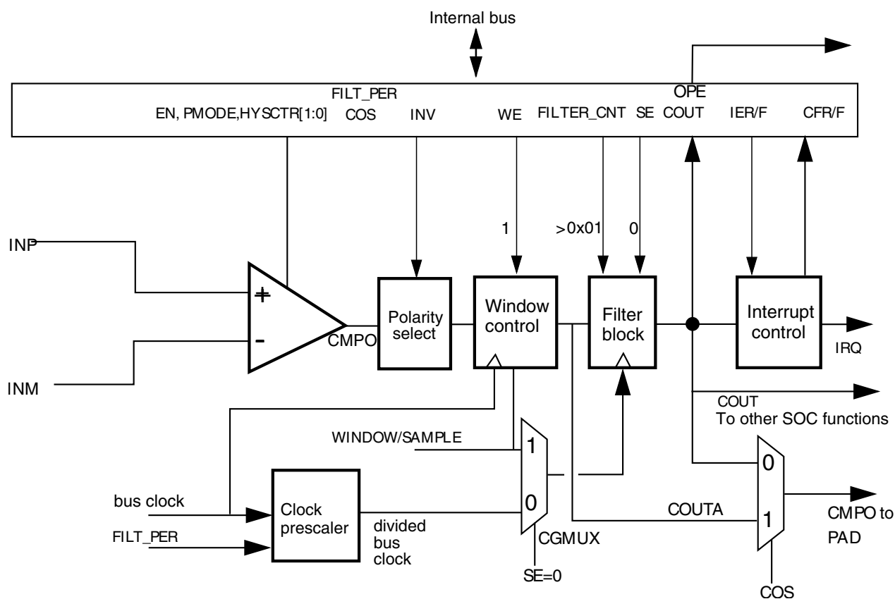
Figure 26-23. Windowed/Filtered mode
