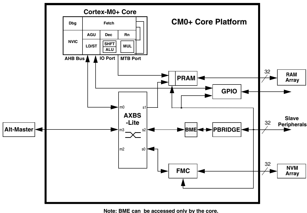
Figure 16-1. Cortex-M0+ core platform block diagram
