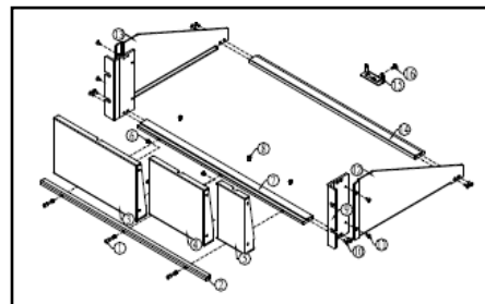
Model 2260B-RMK-EIA: Rack mount kit (EIA racks).
