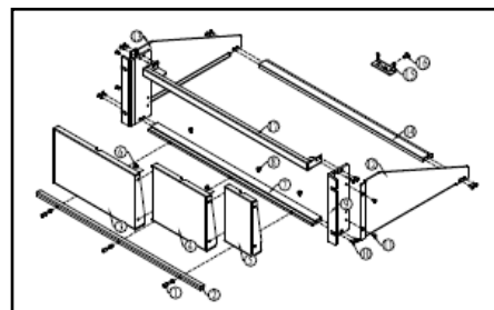
Model 2260B-RMK-JIS: Rack mount kit (JIS racks).
