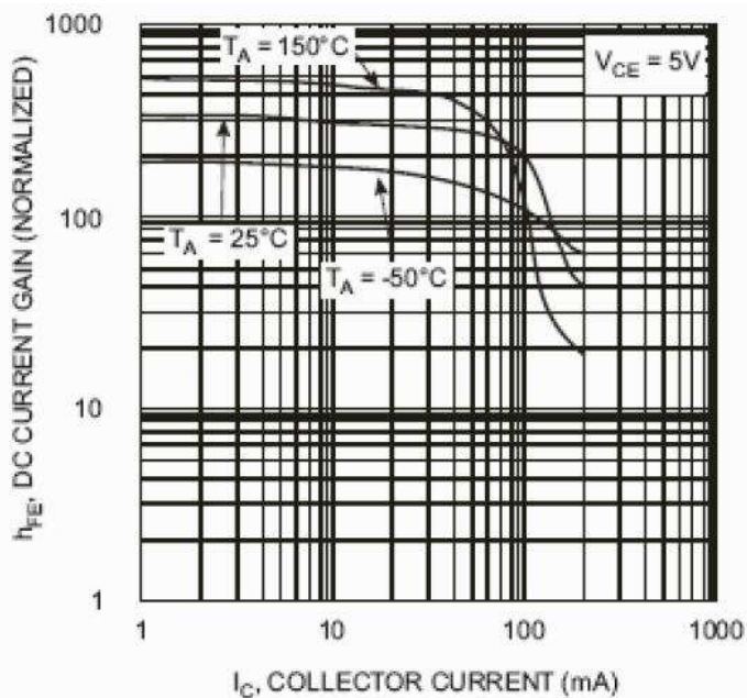
Fig. 3, DC Current Gain vs. Collector Current
