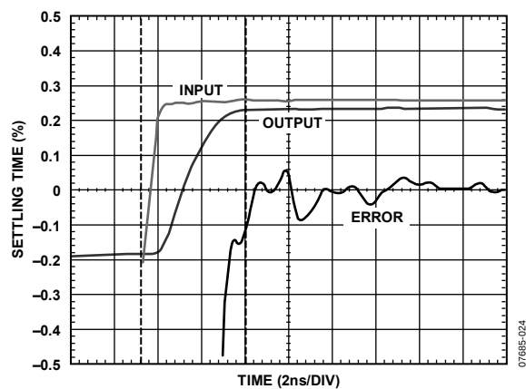
Figure 16. Settling Time
