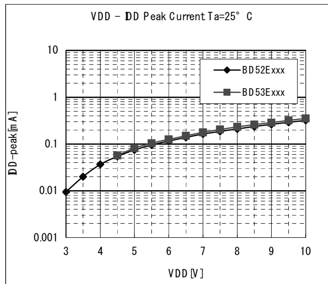
Figure.22 I DD Peak Current vs. Power Supply Voltage
