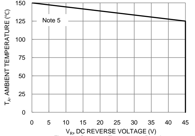
Figure 4. Operating Temperature Derating
