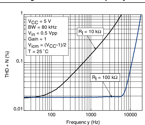
Figure 19. THD+N vs. frequency
