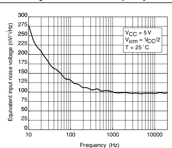
Figure 17. Noise vs. frequency
