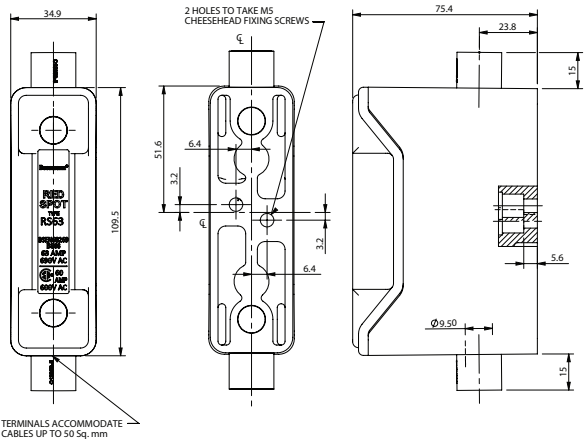
Front connected
