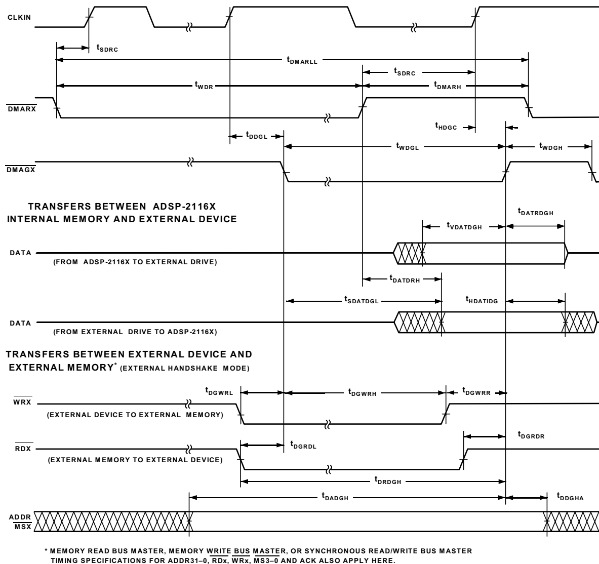
Figure 23. DMA Handshake Timing
