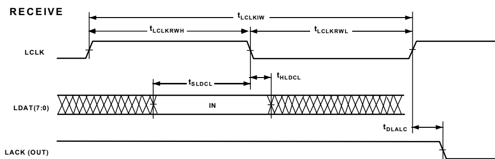
Figure 24. Link Ports—Receive
