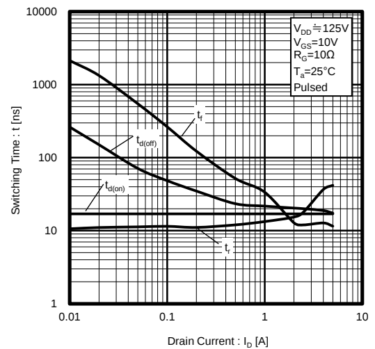
Fig.10 Switching Characteristics
