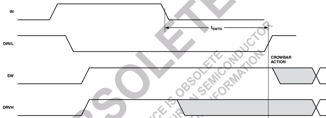
Figure 5. Switching Waveforms—SW Node Failure Mode—DRV_L Timeout
