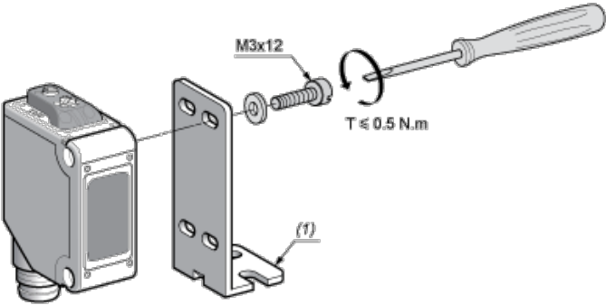
(1) Metal bracket
