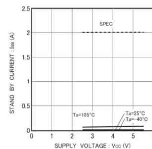
Fig.43 Consumption current at standby action I_{SB}
