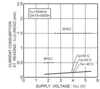
Fig.16 Consumption current at READ action I_{CC2}(\text{READ}, f_{SK}=500\text{kHz})
