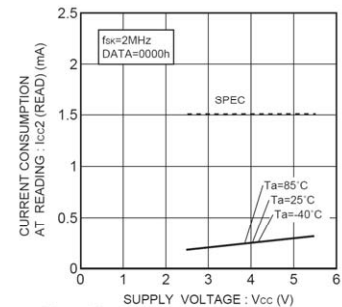
Fig.13 Consumption current at READ action I_{CC2}(\text{READ}, f_{SK}=2\text{MHz})
