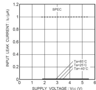
Fig.10 Input leak current I_{IL}(\text{CS,SK,DI})
