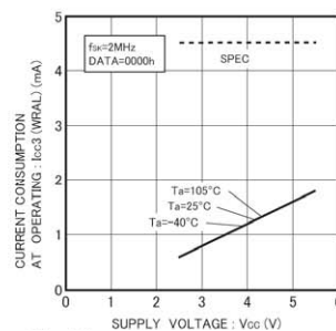
Fig.42 Consumption current at WRAL action I_{CC3}(WRAL, f_{SK}=2MHz)
