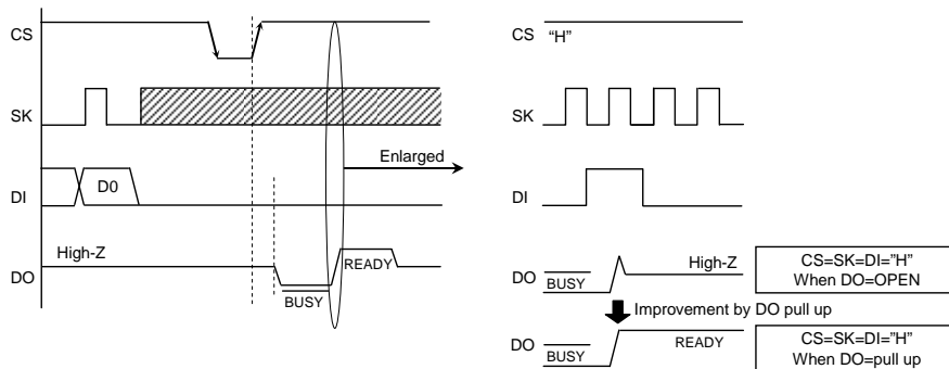
Fig.76 READY output timing at DO=OPEN
