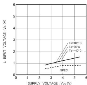
Fig.33 H input voltage V_{IL} (CS,SK,DI)
