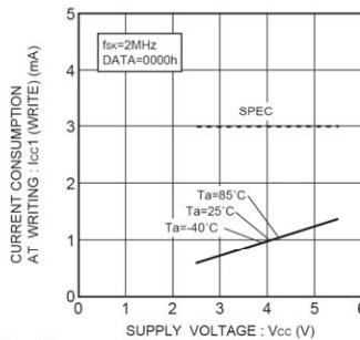
Fig.12 Current consumption at WRITE action I_{CC1}(\text{WRITE}, f_{SK}=2\text{MHz})
