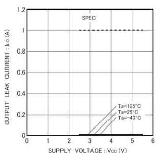
Fig.39 Output leak current I_{LO} (DO)
