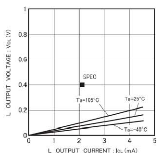
Fig.35 L output voltage V_{OL} - I_{OL} ( V_{CC}=4.0V )
