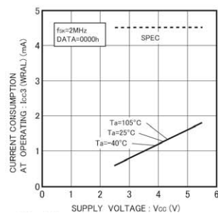
Fig.42 Consumption current at WRAL action I_{CC3} (WRAL, f_{SK}=2MHz )
