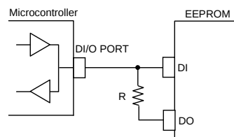
Fig.46 DI, DO control line common connection
