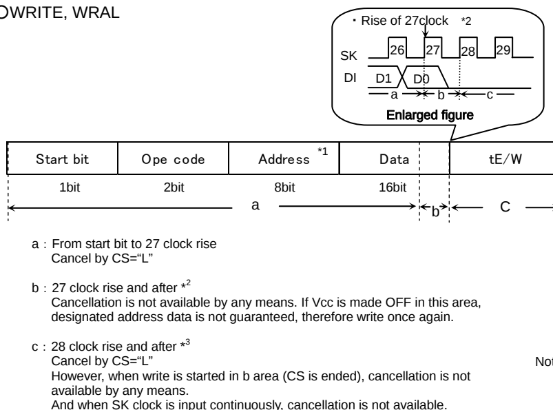
Fig.35 WRITE, WRAL cancel available timing
