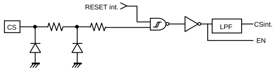
Fig.37 Input circuit (CS)
