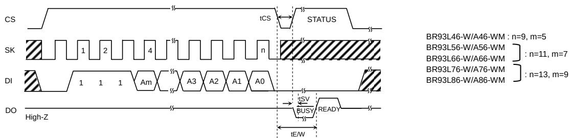
Fig.64 Erase cycle timing
