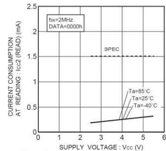
Fig.13 Consumption current at READ action I_{CC2}(\text{READ}, f_{SK}=2\text{MHz})
