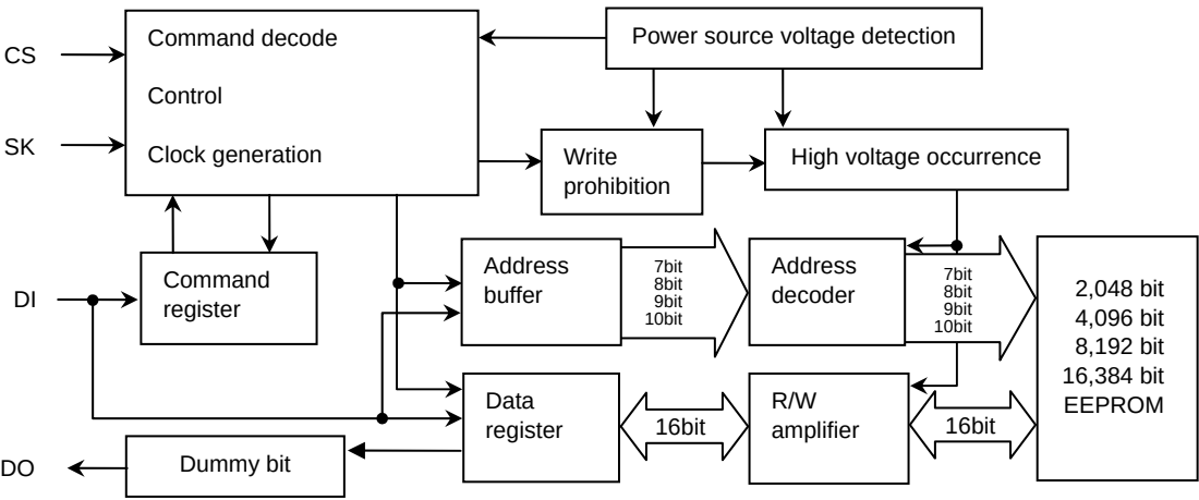
Fig. 27 Block diagram
