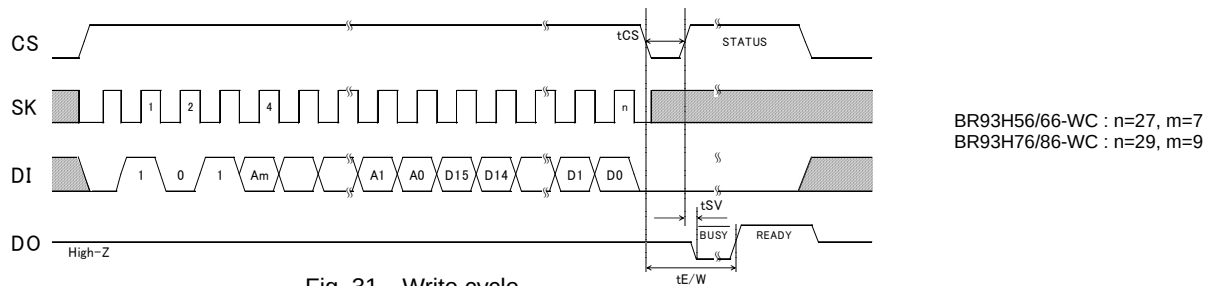
Fig. 31 Write cycle
