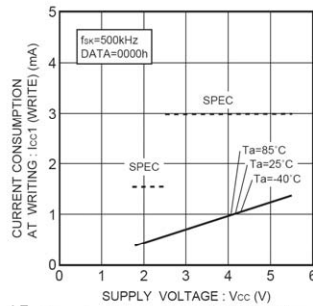
Fig.15 Current consumption at WRITE action I_{CC1}(\text{WRITE}, f_{SK}=500\text{kHz})
