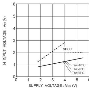
Fig.2 H output voltage V_{IH}(\text{CS,SK,DI})
