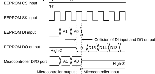
Fig.81 Collision timing at read data output at DI, DO direct connection
