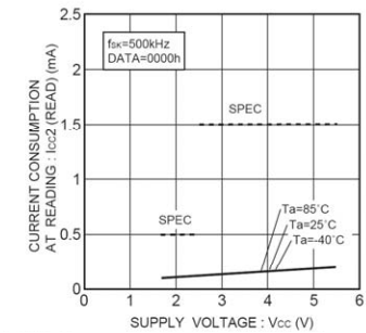
Fig.16 Consumption current at READ action I_{CC2}(\text{READ}, f_{SK}=500\text{kHz})
