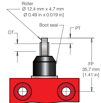
Figure 11. 24CE55 Dimensions
