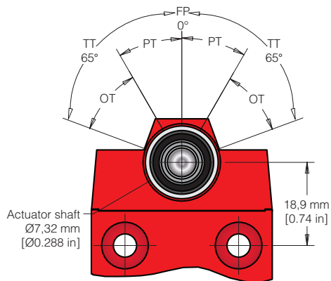
Figure 6. 24CE16 Dimensions
