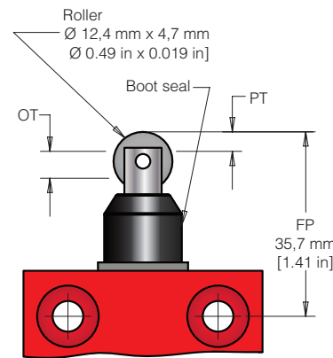
Figure 10. 24CE31 Dimensions
