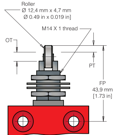
Figure 9. 24CE29 Dimensions
