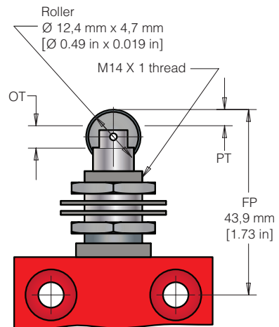
Figure 8. 24CE28 Dimensions
