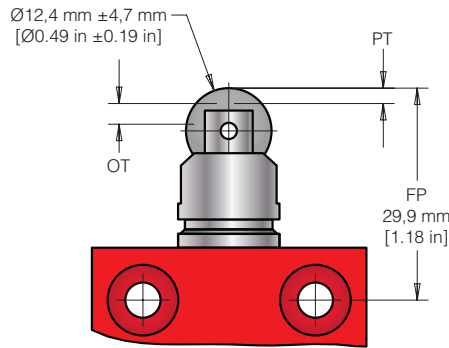
Figure 4. 24CE2 Dimensions
