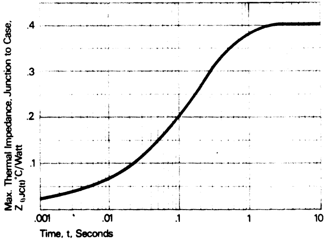
Figure 5. Transient thermal impedance vs. time.
