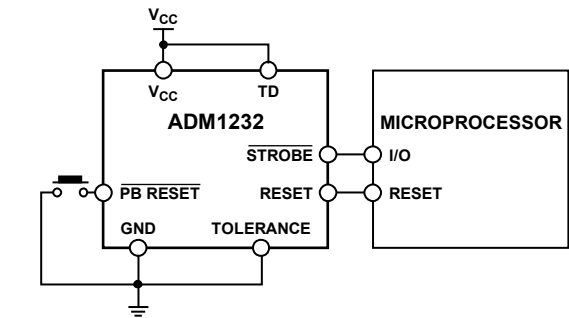
Figure 6. Typical Push-Button Reset Application
