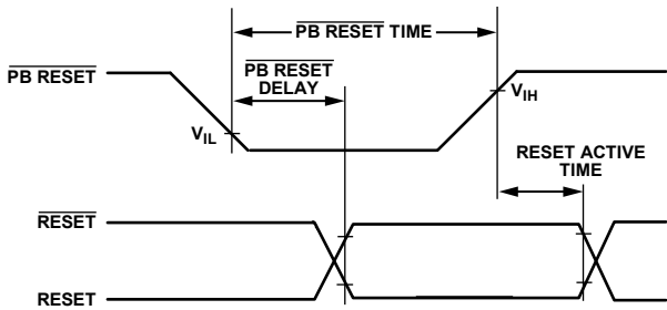
Figure 7. \overline{\text{PB RESET}}
