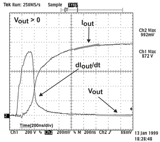
Figure 20. Current and voltage of the ACS during IEC 61000-4-5 standard test with R = 150 \, \Omega , L = 5 \, \mu\text{H} , V_{pp} = 2\text{kV}
