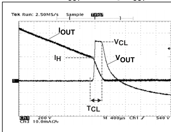
Figure 17. Turn-off operation of the ACS302 with an electro-valve: waveform of the pin OUT current I_{OUT} and voltage V_{OUT}
