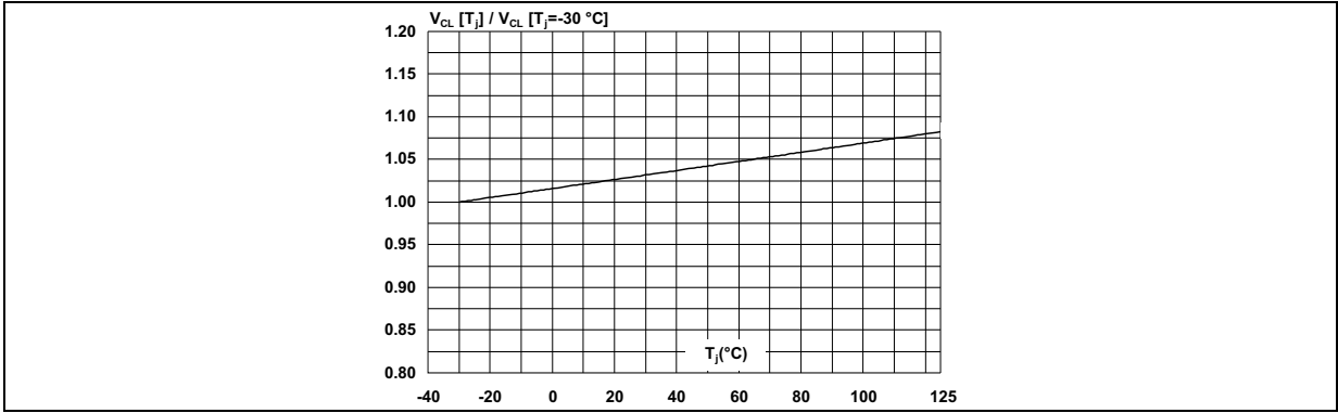
Figure 15. Relative variation of clamping voltage ( V_{CL} ) versus junction temperature (minimum values)
