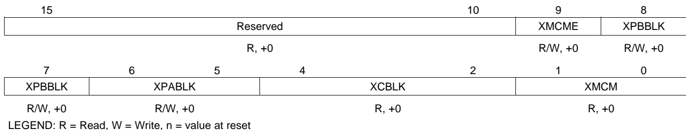
Figure 3-11. Multichannel Control Register 2x (MCR2x)
