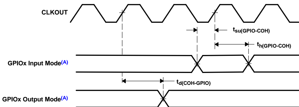
Figure 5-31. GPIOx Timings
