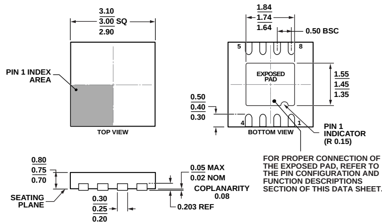
Figure 73. 8-Lead Lead Frame Chip Scale Package [LFCS_P_WD] 3 mm x 3 mm Body, Very Thin, Dual Lead (CP-8-13) Dimensions shown in millimeters
