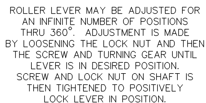
LEVER ADJUSTMENT DETAIL SCALE 2:1
