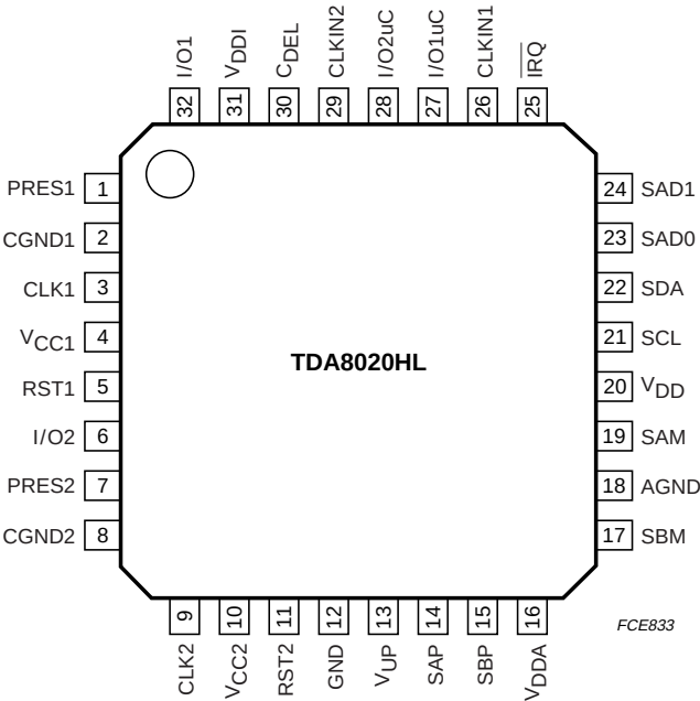
Fig.2 Pin configuration.
