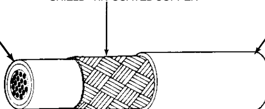
CABLE CONSTRUCTION DETAILS
