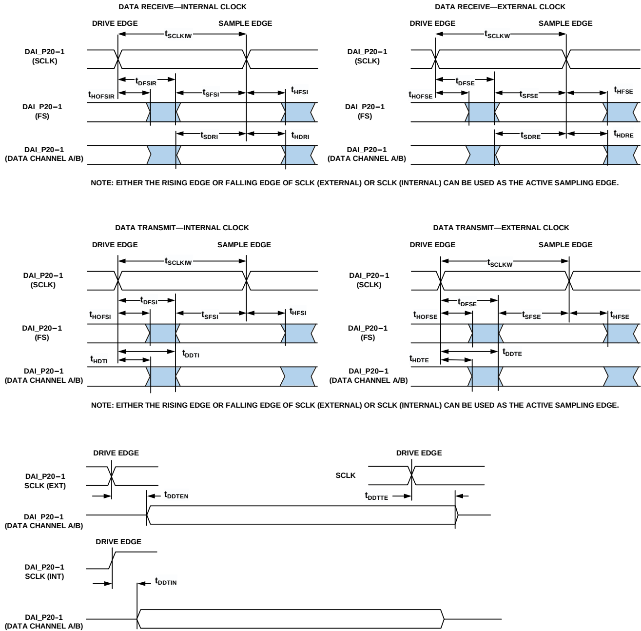
Figure 19. Serial Ports
