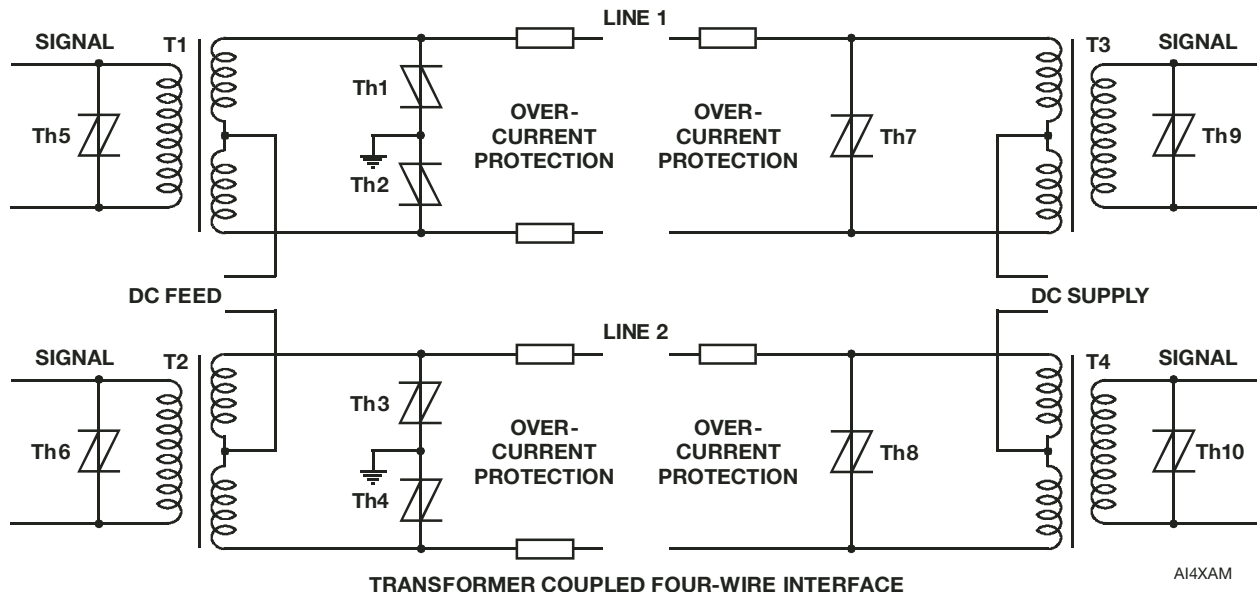
Figure 12. 4-Wire System
