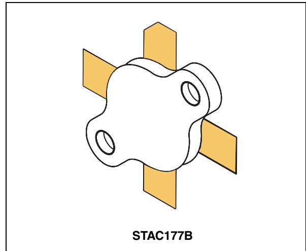
Figure 1. Pin connection
