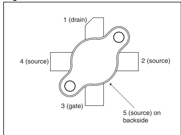
Figure 1. Pin connection
