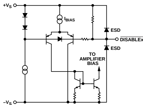
Figure 45. \overline{\text{DISABLEx}} Circuit
