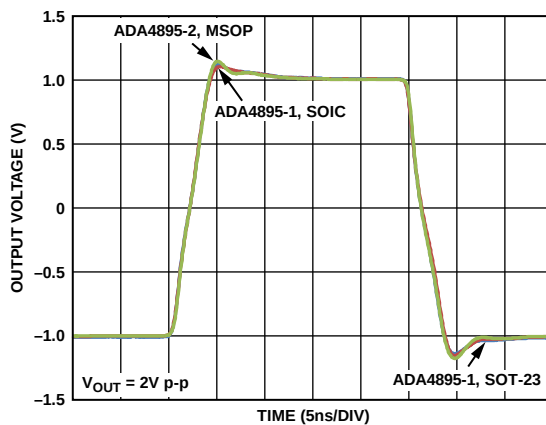
Figure 29. Large Signal Transient Response vs. Package
