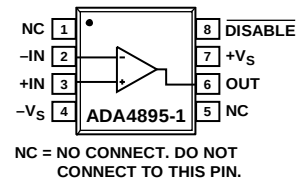
Figure 1. ADA4895-1 Single Amplifier (8-Lead SOIC)
