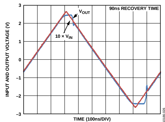
Figure 28. Output Overdrive Recovery Time
