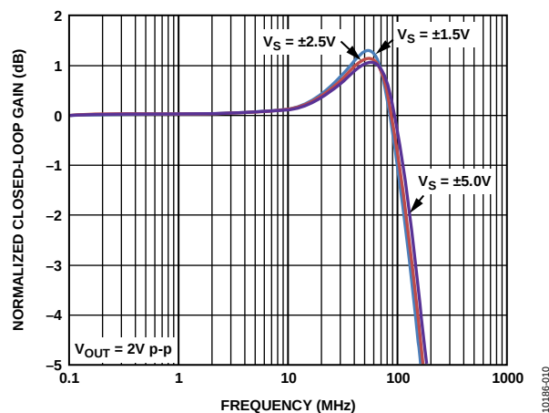
Figure 11. Large Signal Frequency Response vs. Supply Voltage
