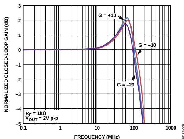
Figure 12. Large Signal Frequency Response vs. Gain
