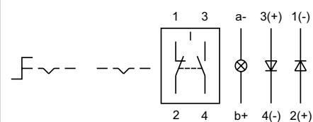
Wiring diagram 21
