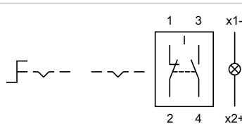
Wiring diagram 22
