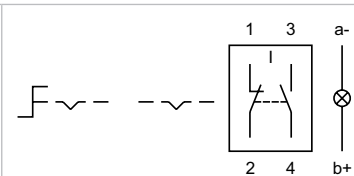
Wiring diagram 23
