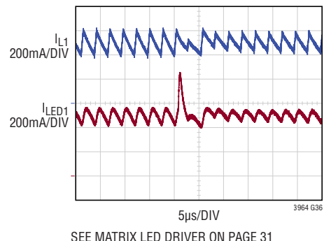
Transient Response at V_{IN} = 34V One LED On to Zero LED On
