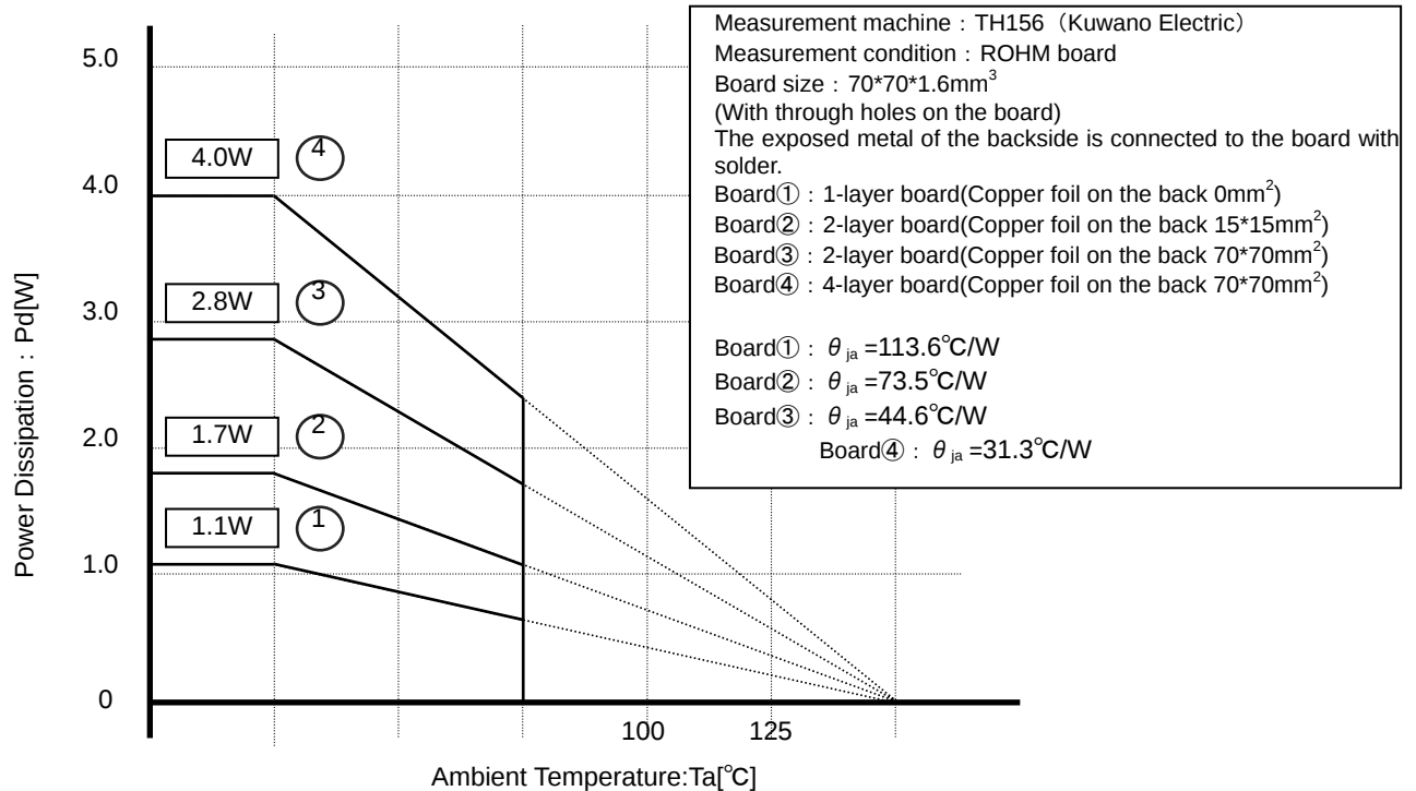
Fig.2 HTSSOP-B24 Derating curve
