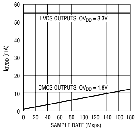
LTC2231: I_{OVD} vs Sample Rate, 5MHz Sine Wave Input, -1\text{dB}
