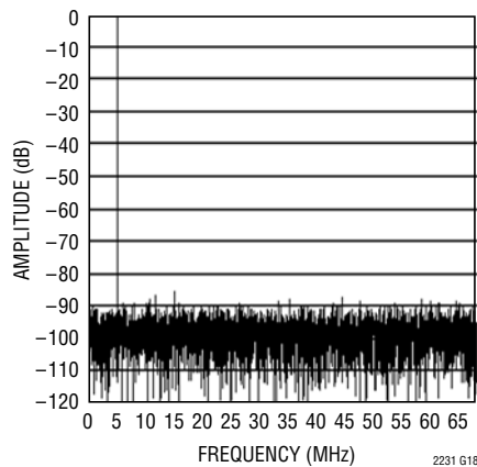
LTC2231: 8192 Point FFT, f_{IN} = 140\text{MHz} , -1dB, 2V Range
