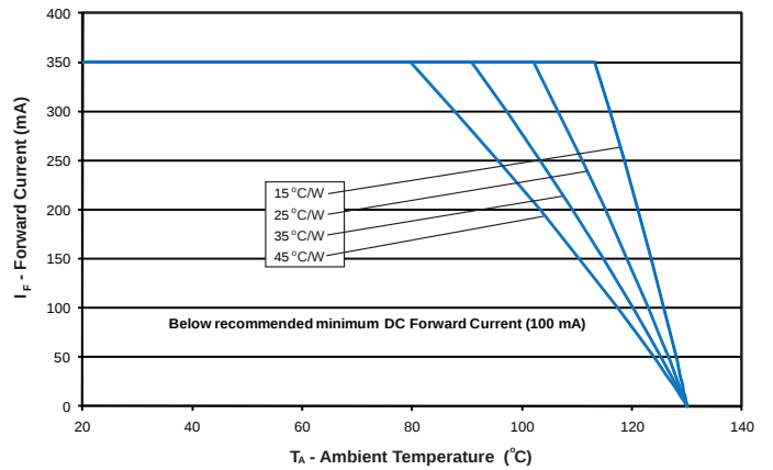
Figure 18. Maximum forward current vs. ambient temperature, based on T_{JMAX} = 130^{\circ}\text{C} , PC amber LXM2-PL01 emitters.
