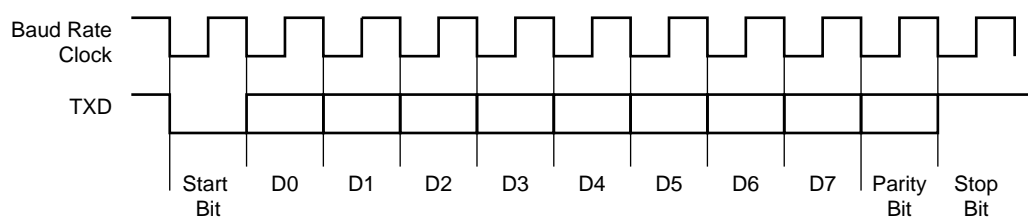
Figure 39-6. Character Transmit
