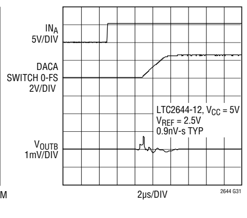
DAC-to-DAC Crosstalk (Dynamic)
