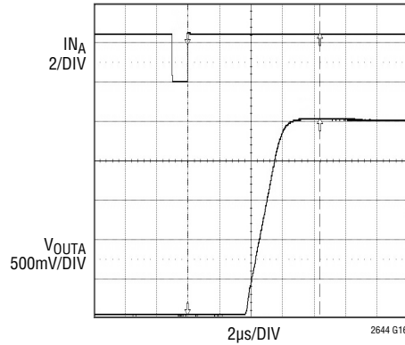
IN_X to V_{OUTX} Delay Full-Scale Transition
