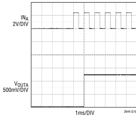
Exiting Idle Mode Zero-Scale to Mid-Scale (IDLSEL=GND)
