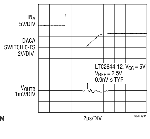
DAC-to-DAC Crosstalk (Dynamic)
