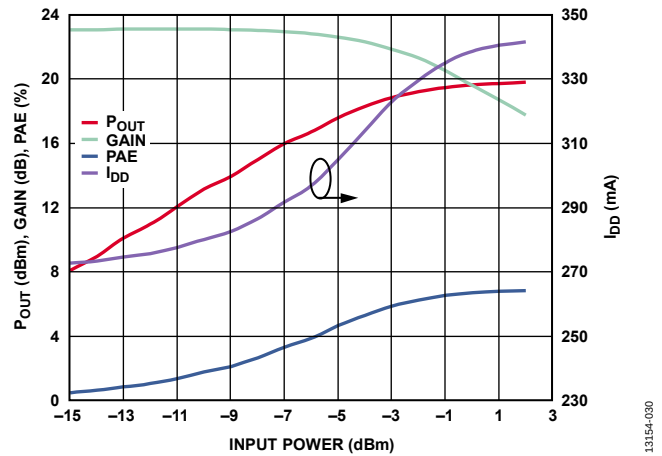
Figure 33. P_{OUT} , Gain, PAE, and I_{DD} vs. Input Power, V_{CTL1}/V_{CTL2} = -5 V, RF = 86 GHz
