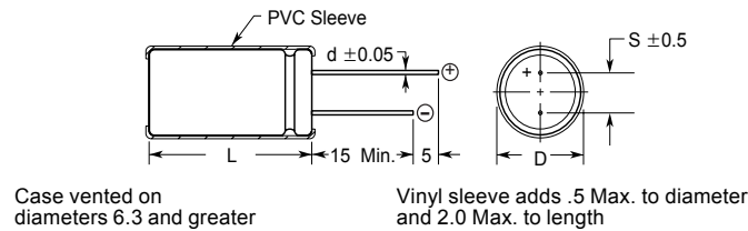
Outline Dimensions (Millimeters)
